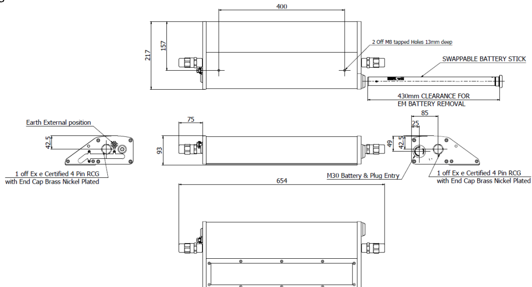
Fig. 1 Sealed For Life version PRB/05L/LE/EM/**/SFL shown for illustration
