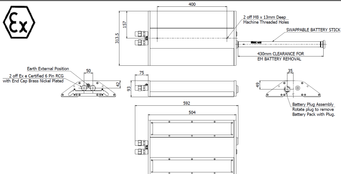
Fig. 1 Sealed For Life version PRB/05L/LE/EM/**/SFL shown for illustration
